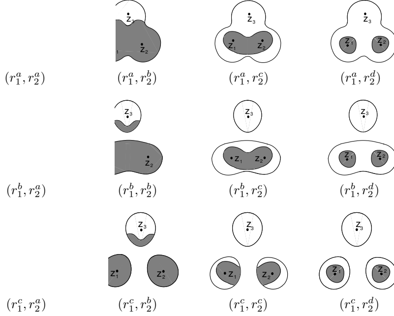
FIGURE 7. The region D_{q,p} defined in Theorem 4.1 is given by D_{q,p} = O_p \cap B_{q,p} , where O_p is the "lemniscate domain" of foci z_1, \dots, z_p and parameter r_1 . Also, B_{q,p} \equiv \{z \in \mathcal{C}, \prod_{k=1}^q |(z - z_k)|^{m_k} < r_2 \prod_{k=q+1}^p |(z - z_k)|^{m_k}\} . These pictures show the topologically different forms of D_{q,p} depending on the relative value of r_1 and r_2 when q = 2 and p = 3 . The pictures are labeled with (r_1, r_2) . In these pictures z_1 |z_1 - z_2| < |z_1 - z_3|, |z_2 - z_3| and r_2^a > r_2^b > r_2^c > r_2^d .
