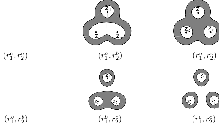
FIGURE 5. Shape of the "lemniscate annulus" A_p for p = 3 . It depends on the relative size of the parameters r_1 and r_2 defined in (3.8). The different forms are labeled by (r_1, r_2) with r_1 > r_2 . In these pictures |z_2 - z_3| < |z_1 - z_3| , |z_1 - z_2| and r_2^a > r_2^b > r_2^c .
